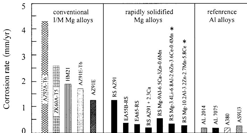
Fig. 12 Corrosion rate of light alloys obtained by weight loss measurements in 5% NaCl solution. * Data from electrochemical impedance spectroscopy. (Reprinted, by permission from Ref. 61. Copyright © 1996 by Wiley-VCH.)
