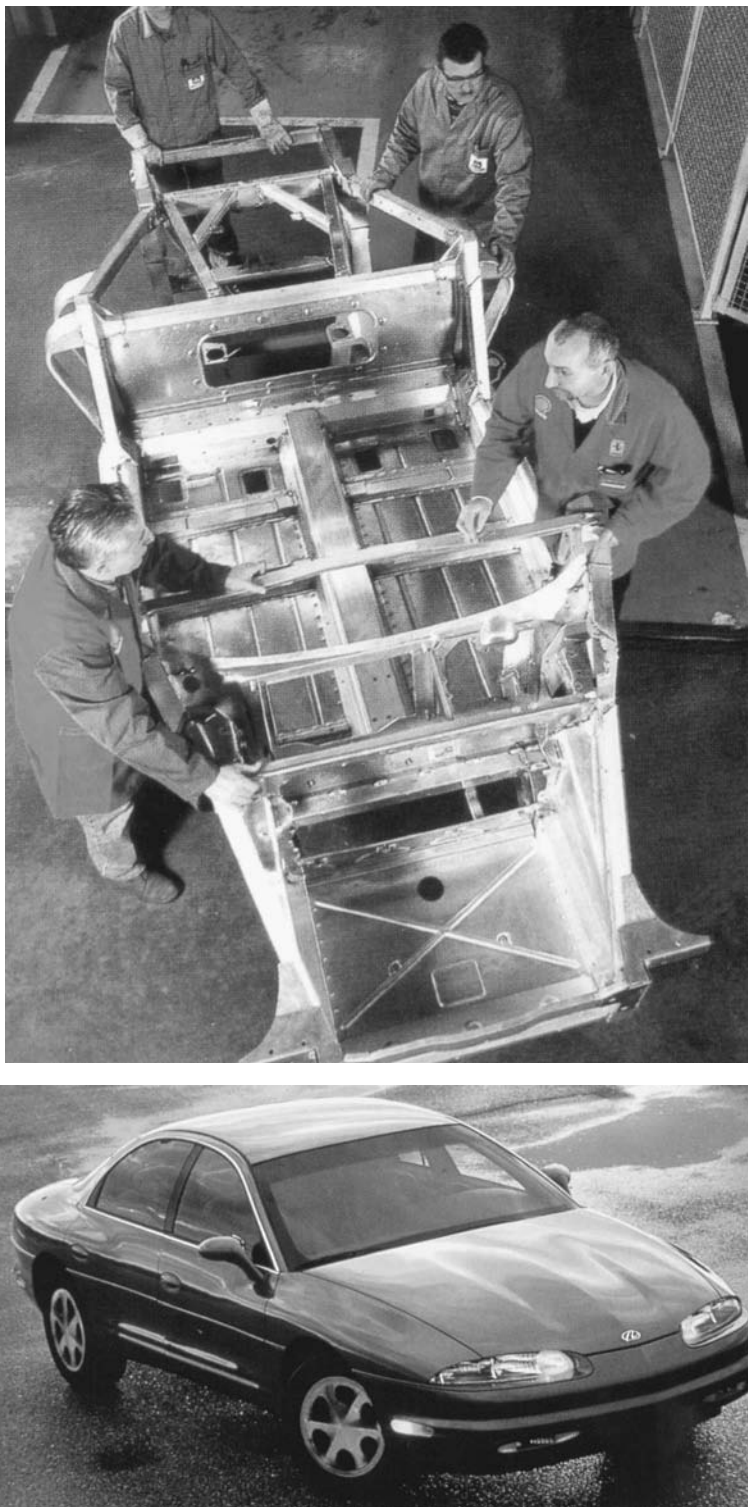
Fig. 13 Automotive structures are likely to employ increasing amounts of 5754-O formed sheet for parts such as internal door stiffeners or (a) the entire body in white; (b) external body panels are more likely to be higher strength 6111-T4.
