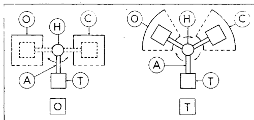
Fig. 21 Swing/rotary arm rotational molding: [O], one-arm (swing); [T], three-arm (rotary); O, oven; H, hub; C, cooling chamber; T, mold; A, arm. (From Charrier, J.-M., Polymeric Materials and Processing: Plastics, Elastomers and Composites , Hanser Publishers, Munich, 1990.)
