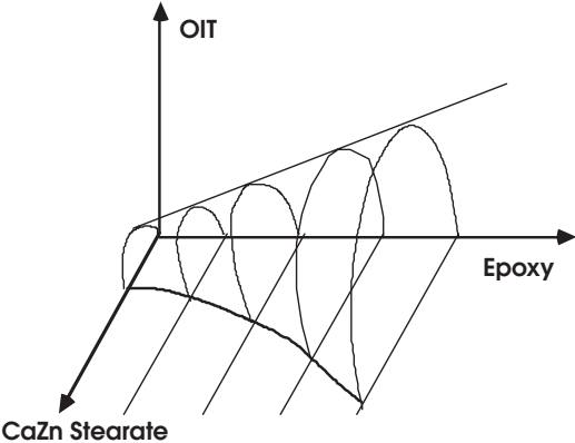
Fig. 2 Three-dimensional schematic of PVC stability.
