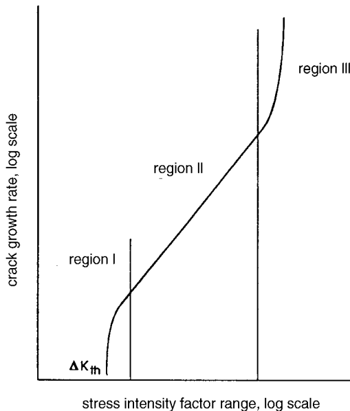
Fig. 25 Schematic representation of fatigue crack growth rate data.
