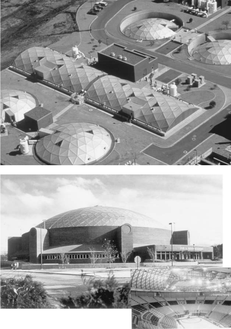
Fig. 8 Sheet of 5xxx alloys often forms the surface of geodesic dome structures, as in these examples of (a) a water treatment plant and (b) a wide-span arena roof. The structural supports are typically 6061 or 6063 extruded shapes or tubular members.
