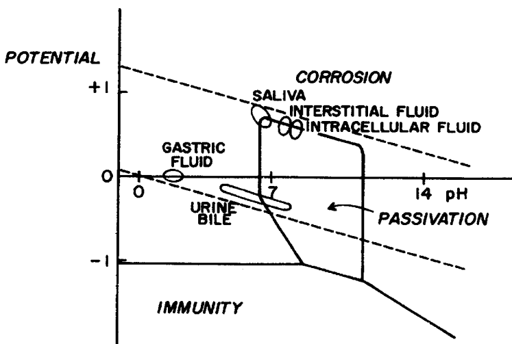
Fig. 5 Pourbaix diagram for chromium in aqueous solution of 1 N Cl^- . The diagram indicates the electrochemical environment of various regions of the body. [From John H. Dumbleton and Jonathan Black, An Introduction to Orthopaedic Materials , Thomas Publishing, Springfield, IL, 1975, with permission].
