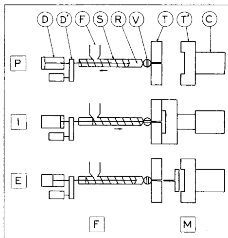
Fig. 28 Injection-molding principle: [F], feed unit; [M], mold unit; [P], plastication stage; [I], injection;; [E], product ejection (demolding); D, axial screw drive; D', rotation screw drive; F, feed hopper; S, reciprocating screw; R, material “reservoir”; V, valve; T, T', mold halves; C, mold clamping device. (From Charrier, J.-M., Polymeric Materials and Processing: Plastics, Elastomers and Composites , Hanser Publishers, Munich, 1990.)
