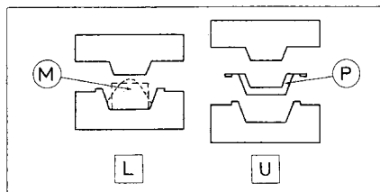
Fig. 25 Flash molding: [L], loading; [U], unloading; M, material charge; P, product. (From Charrier, J.-M., Polymeric Materials and Processing: Plastics, Elastomers and Composites , Hanser Publishers, Munich, 1990.)
