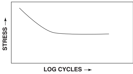
Typical Fatigue Curve at Low Temperature
