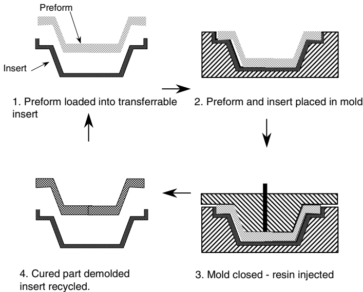
Fig. 29 Productivity in the RTM process may be enhanced by use of a system of transferable mold inserts. These are auxiliary tools, usually thin sheet metal construction. The preforms are built up on these inserts, which are finally placed into the RTM molds. Several inserts may be rotated, so that preform assembly and demolding may be carried out concurrently with molding.
