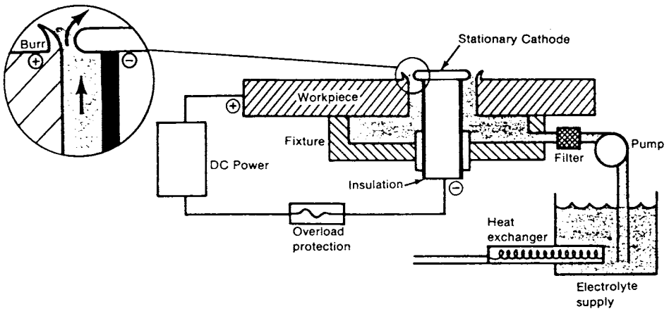
Fig. 39 Electrochemical deburring.
