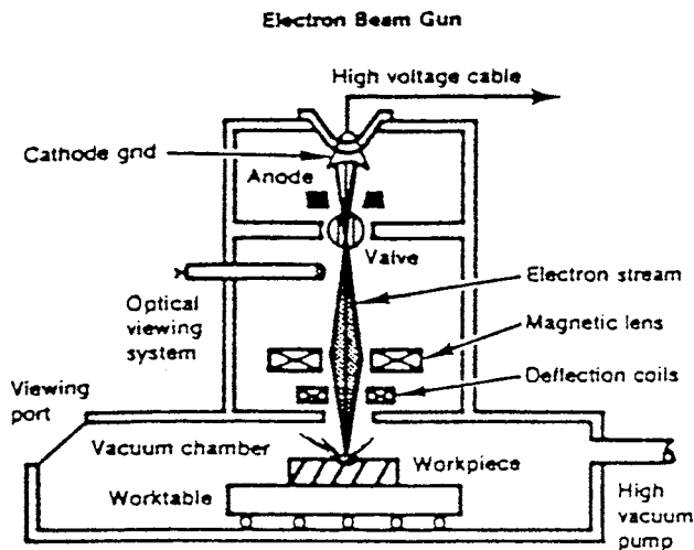
Fig. 49 Electron-beam machining.
