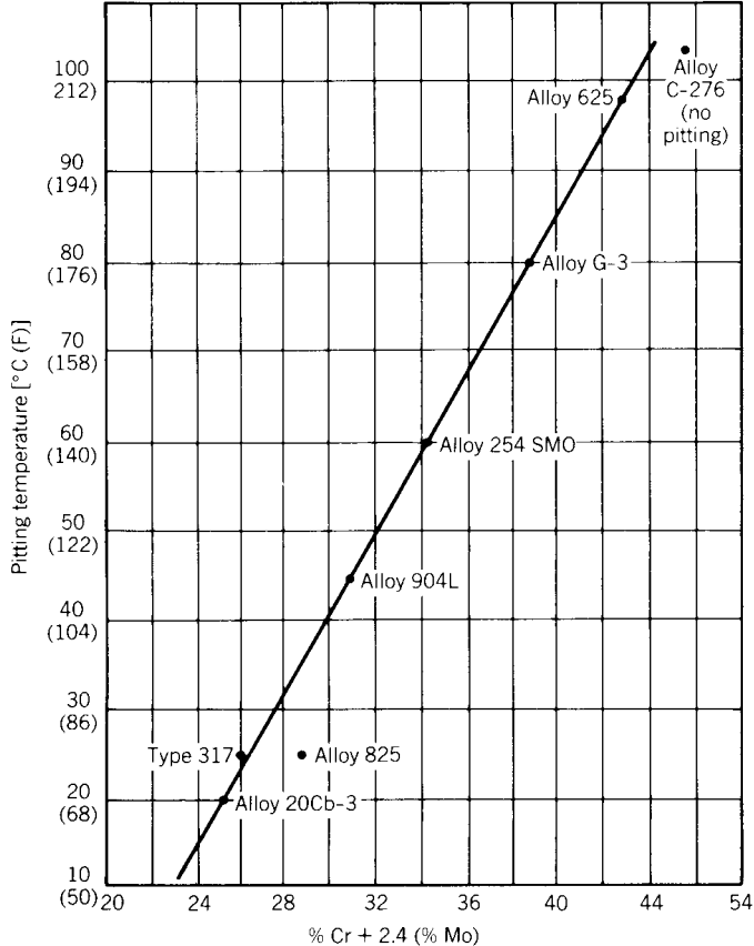
Fig. 4 Critical temperature for pitting in 4% NaCl + 1% Fe 2 (SO 4 ) 3 + 0.01 M HCl versus composition for Fe–Ni–Cr–Mo alloys.
