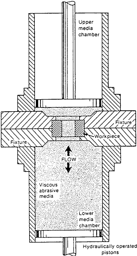
Fig. 31 Abrasive flow machining.
