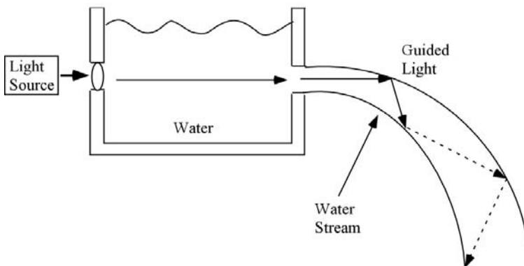
Fig. 10 Light guided down a water stream demonstrating principle of internal reflection of light.
