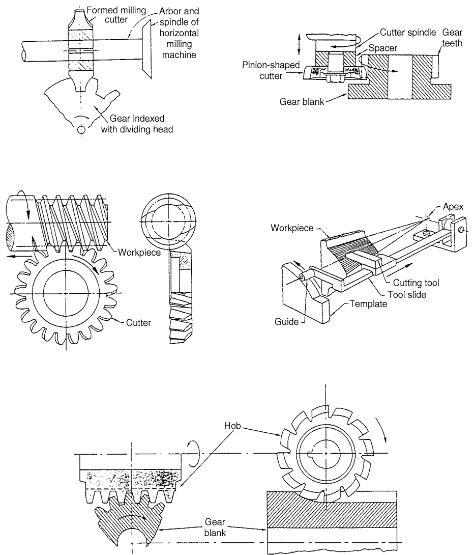
Fig. 23 Machining gears.
