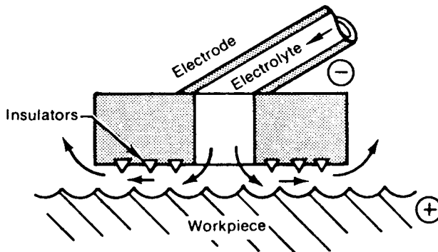
Fig. 45 Electrochemical sharpening.
