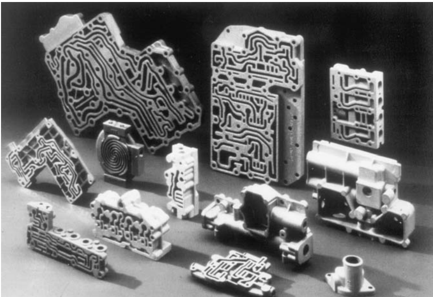
Fig. 16 Complex 3xx.x castings made by the investment casting processes provide the ability to obtain exceptionally intricate detail and fine quality.
