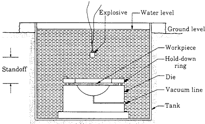
Fig. 17 High-energy-rate forming.
