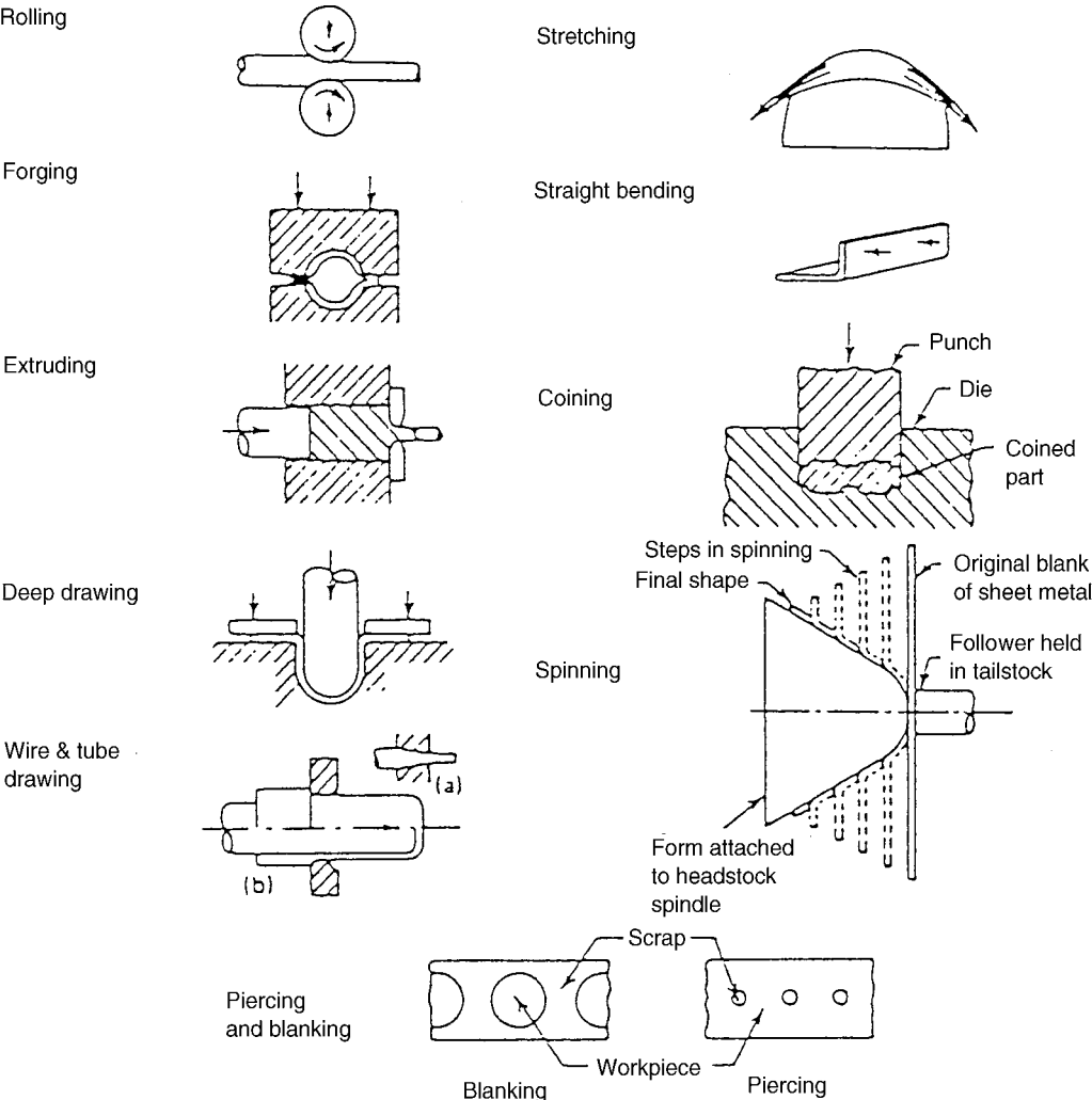
Fig. 1 Metal-forming processes.
