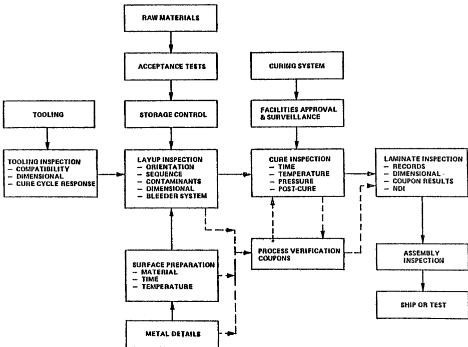
Fig. 5 Inspection requirements for flight-critical structure.
