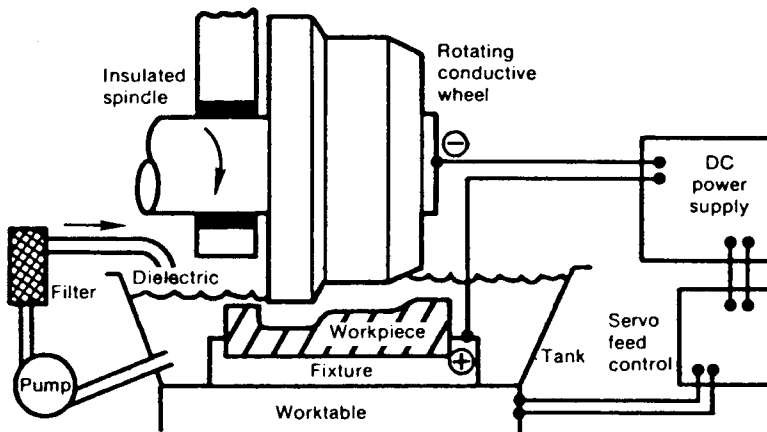
Fig. 50 Electrical discharge grinding.
