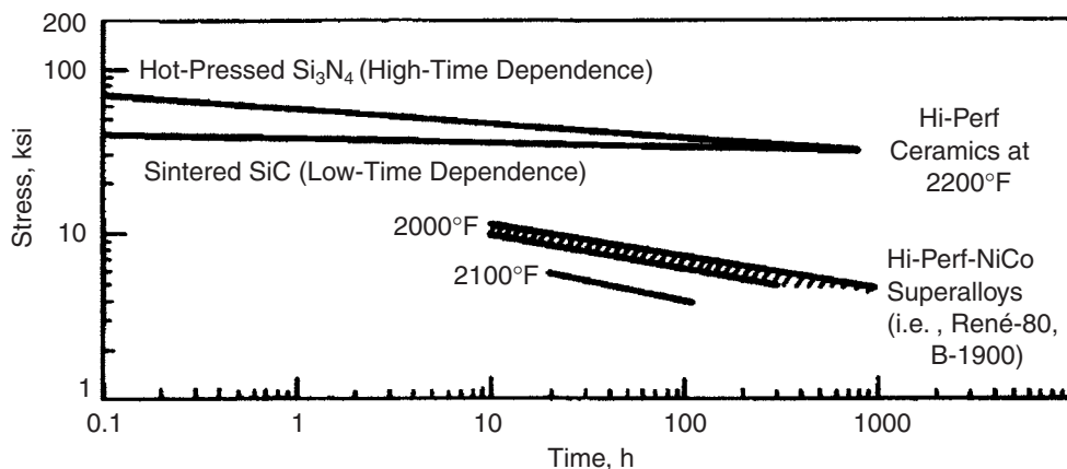
Fig. 2 Stress rupture performance of nonoxide structural ceramics compared to superalloys (oxidizing atmosphere).
