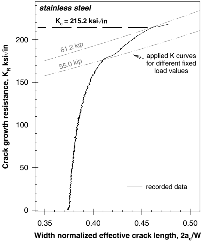
Fig. 12 Example R curve from a K_{IC} fracture toughness test performed on stainless steel.
