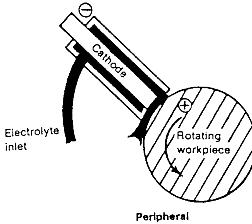
Fig. 46 Electrochemical turning.
