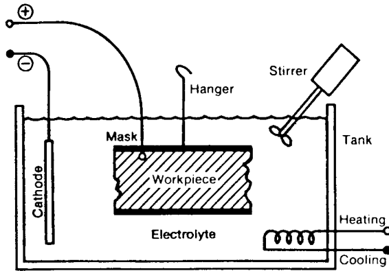
Fig. 58 Electropolishing.
