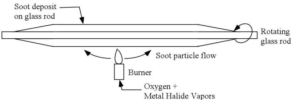
Fig. 12 Soot deposition onto a rotating rod by the outside vapor deposition (OVD) process.
