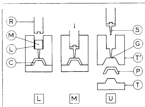
Fig. 27 Pot transfer molding: [L], loading; [M], molding; [U], unloading; C, cavity; L, pot; M, material charge; R, transfer piston; S, sprue (scrap); G, gate; T, T', mold halves; P, product. (From Charrier, J.-M., Polymeric Materials and Processing: Plastics, Elastomers and Composites , Hanser Publishers, Munich, 1990.)
