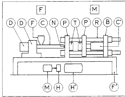
Fig. 29 Injection-molding machine: [F] , feed unit; [M] , mold unit; D , axial screw drive; D' , rotation screw drive; F , feed hopper; C , plastification/injection cylinder; P , stationary platen; T , mold; P' , moving platen; R , tie bars; B , back platen; C' , mold clamping mechanism; F' , machining frame; H' , hydraulic accumulator; H , hydraulic pump; M , electric motor; In , injection unit. (From Charrier, J.-M., Polymeric Materials and Processing: Plastics, Elastomers and Composites , Hanser Publishers, Munich, 1990.)
