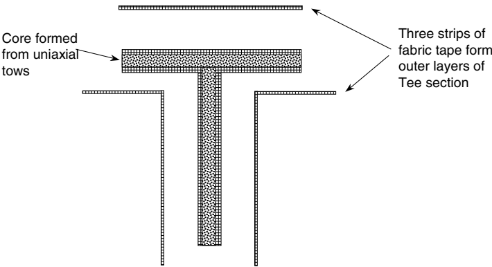
Fig. 37 Pultruded sections may be assembled from a variety of tow and tape reinforcements. This is illustrated for a Tee section formed from uniaxial tows in the core and three fabric tapes. These could be of either woven fabric or random mat.
