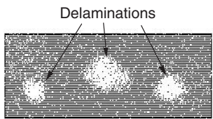
Fig. 11 Typical C-scan image of a composite specimen showing delaminations and porosity. Black and white are reversed.
