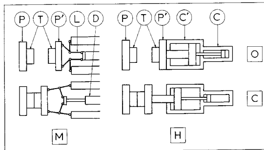
Fig. 30 Mold-clamping mechanisms: [M] , mechanical (double toggle); [H] , hydraulic (dual cylinder); [O] , mold open configuration; [C] , mold closed configuration; P , stationary platen; T , mold; P' , moving platen; L , link; D , toggle drive; C' , lock cylinder; C , traverse cylinder. (From Charrier, J.-M., Polymeric Materials and Processing: Plastics, Elastomers and Composites , Hanser Publishers, Munich, 1990.)
