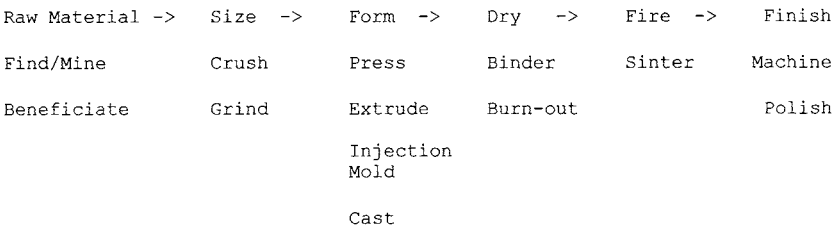
Fig. 3 Unit operations in manufacturing ceramic part.
