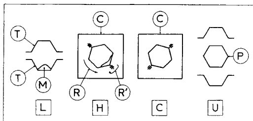
Fig. 19 Rotational molding process: [L], loading; [H], heating; [C], cooling; [U], unloading; T, T', mold halves; M, material charge; R, R', axes of rotation; C, conditioning chamber; P, product. (From Charrier, J.-M., Polymeric Materials and Processing: Plastics, Elastomers and Composites , Hanser Publishers, Munich, 1990.)
