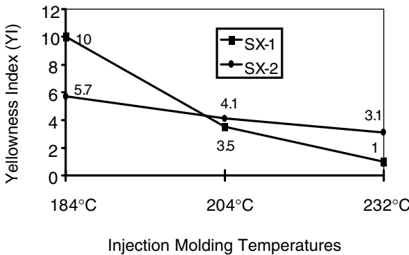
Fig. 23 Clarity of PP pellets improves (YI) as injection-molding temperature increases.
