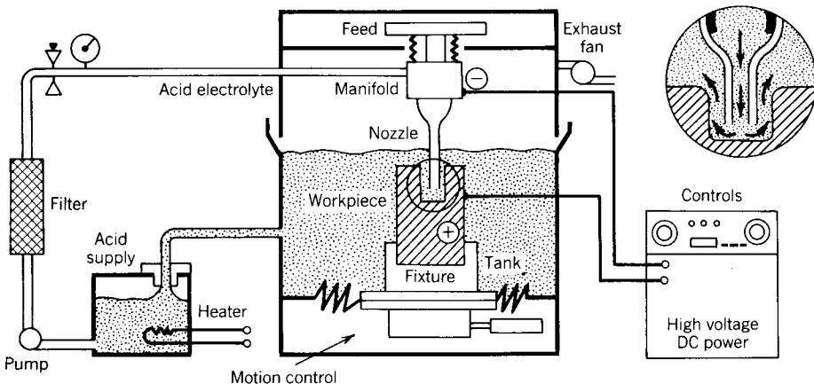
Fig. 47 Electro-stream.
