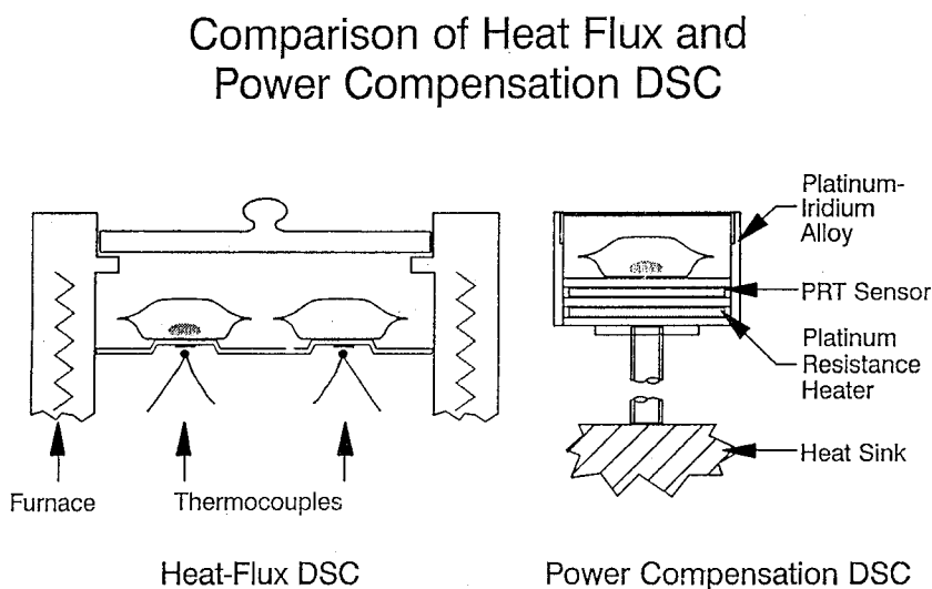
Fig. 6 Two most common types of DSC measuring cells. (Courtesy Perkin-Elmer Corporation)
