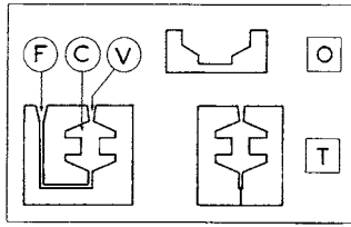
Fig. 22 Casting molds: [O], open mold; [T], two-piece mold; F, feed runner; C, cavity; V, vent. (From Charrier, J.-M., Polymeric Materials and Processing: Plastics, Elastomers and Composites , Hanser Publishers, Munich, 1990.)
