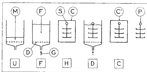
Fig. 18 Fluidized-bed dip coating: [U], unfluidized bed; [F], fluidized bed; [H], substrate heating; [D], dipping; [C], conditioning; M, powdered coating material; F, fluidized particles; D, porous diaphragm; G, gas inlet; S, substrate; C, heating chamber; C', conditioning chamber; P, product. (From Charrier, J.-M., Polymeric Materials and Processing: Plastics, Elastomers and Composites , Hanser Publishers, Munich, 1990.)
