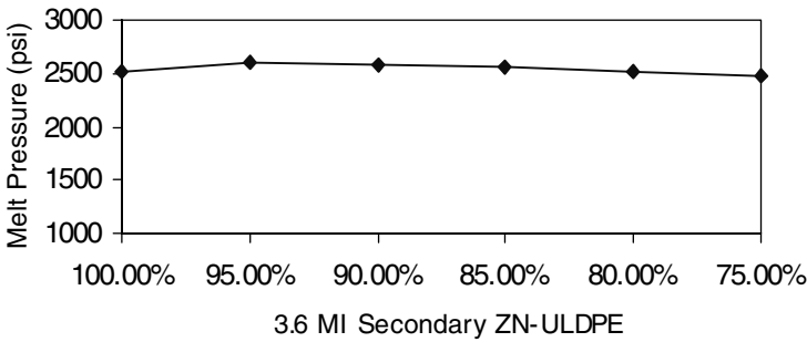
Fig. 22 Melt pressure of 1. O MI m-ULDP and 3. 6 MI ZN ULDPO blends.
