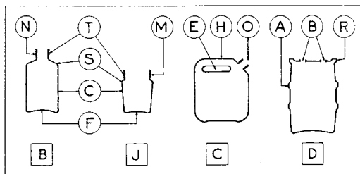
Fig. 15 Blow-molded products: [B], bottle; [J], jar; [C], canister; [D], drum; N, narrow neck; T, thread; S, shoulder; C, body; F, base; M, wide mouth; E, eye; H, handle; O, off-center neck; A, annular rib; B, bungs; R, ring. (From Charrier, J.-M., Polymeric Materials and Processing: Plastics, Elastomers and Composites , Hanser Publishers, Munich, 1990.)
