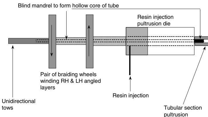
Fig. 39 Further possibilities are to filament wind, using braiding wheels, onto core sections formed from uniaxial or fabric reinforcements. The linear nature of the process allows for any number of operations before the section enters the die.
