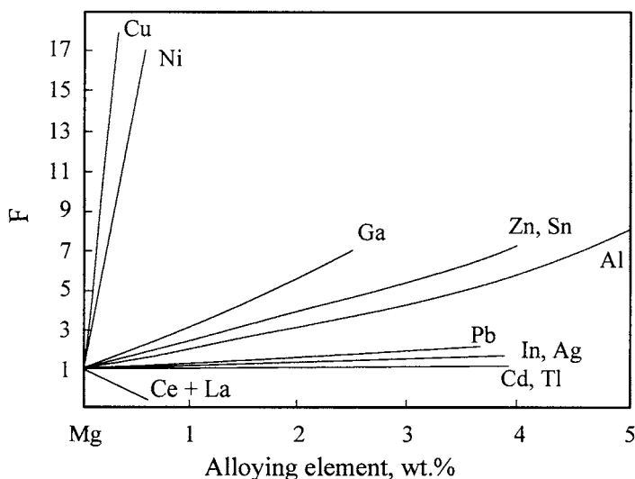
Fig. 4 Effect of alloying elements on the oxidation of Mg at \sim 475^\circ\text{C} (after Ref. 22, values from Ref. 17).
