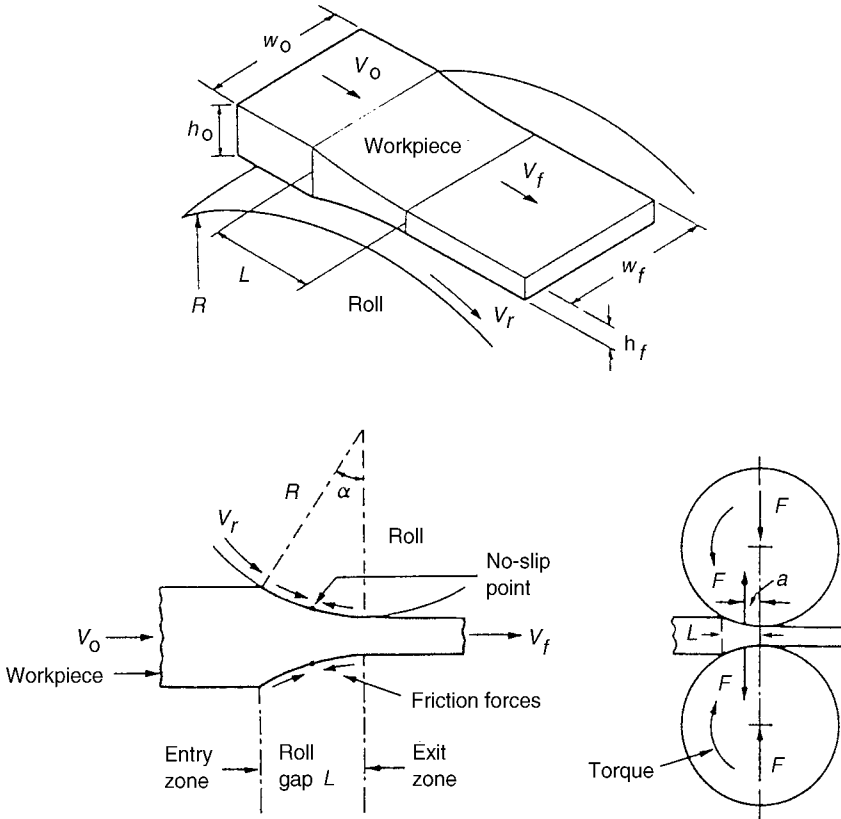
Fig. 2 Hot rolling.
