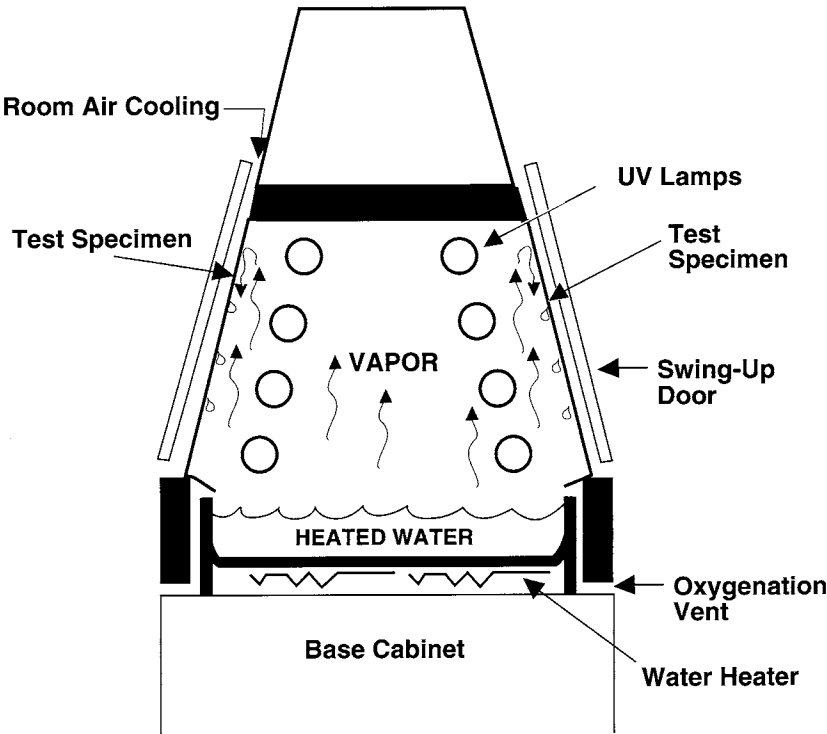
Fig. 21 Cross section of a UV light and condensation apparatus. (Courtesy Q-Panel Lab Products)
