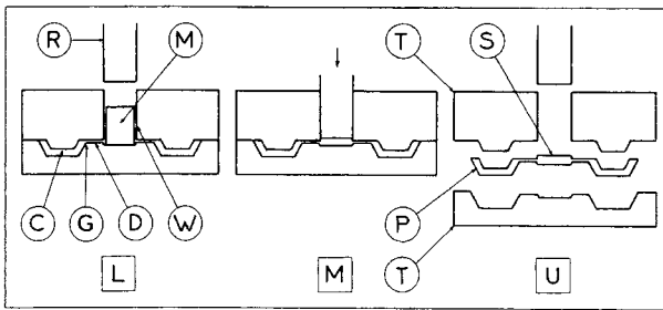
Fig. 26 Plunger transfer molding: [L], loading; [M], molding; [U], unloading; W, loading well; D, distributing channel; G, gate; C, cavity; R, plunger; M, material charge; T', stationary mold half; S, cull (scrap); P, product; T, moving mold half. (From Charrier, J.-M., Polymeric Materials and Processing: Plastics, Elastomers and Composites , Hanser Publishers, Munich, 1990.)
