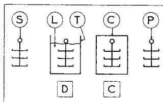
Fig. 17 Liquid dip coating: [D], dipping; [C], conditioning; S, substrate; L, coating liquid; T, tank; C, conditioning chamber; P, product. (From Charrier, J.-M., Polymeric Materials and Processing: Plastics, Elastomers and Composites , Hanser Publishers, Munich, 1990.)
