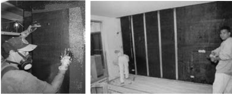
Fig. 10 Applications of composites for strengthening reinforced concrete shear walls. [Courtesy of Structural Composites Construction Inc. (SCCI)]
