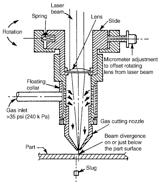
Fig. 55 Laser-beam torch.
