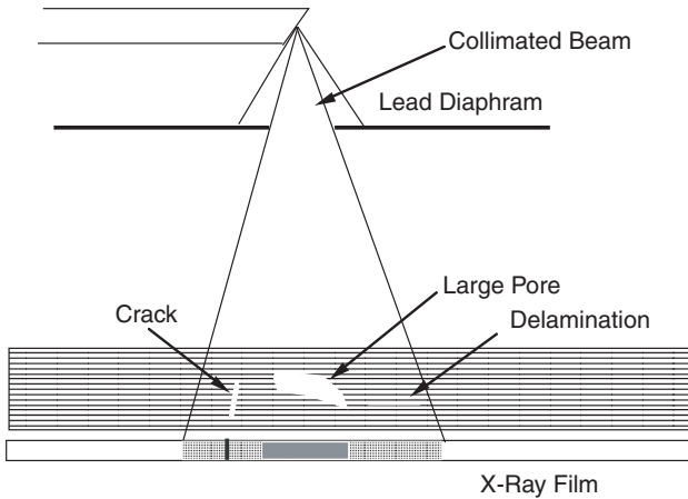
Fig. 12 Schematic radiograph of a typical composite with typical flaws.
