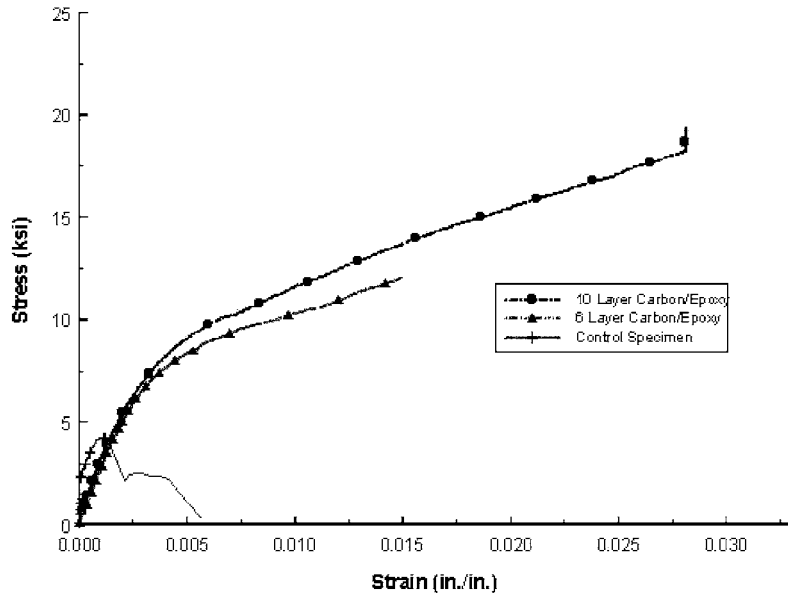
Fig. 31 Experimental stress–strain curves for confined with FRP and unconfined circular columns (Youssef, 2001).
