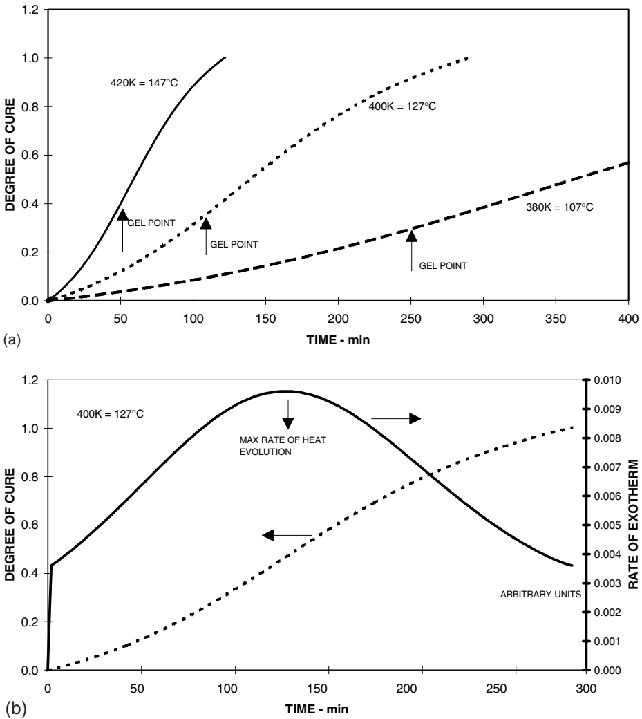
Fig. 7 These figures illustrate the cure characteristics of a typical thermosetting resin, e.g., an epoxy. (a) Shows the cure profile at three different curing temperatures. The degree of cure is plotted against time of cure. The cure rate is much faster at the higher temperatures. A temperature increase of only 20°C, from 107°C to 127°C, reduces the gel time from 250 min to just over 100 min. (b) Cure profile at 127°C is shown together with the rate of exotherm. This peaks soon after gelation. The exotherm rate is higher at higher cure temperatures (not shown). (c) Resin viscosity profiles for the same resin at the three temperatures is shown. The viscosity increases sharply after the gel point and this defines the workable range, or process window .
