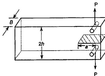
Fig. 9 Double-cantilever beam test method. (From Ref. 14 ASM Handbook, Vol. 8: Mechanical Testing and Evaluation , ASM International, Materials Park, OH 44073-0002.)
