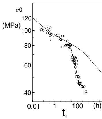
Fig. 14 Lifetime as a function of the (elastically calculated) outer fiber bending stress for static bending tests on \text{Al}_2\text{O}_3 with 4% glass content. Solid line predictions from subcritical crack growth.
