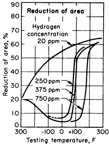
Fig. 5 Ductility of alpha titanium versus test temperature, showing embrittling effects of hydrogen. (From Titanium: A Technical Guide , 1st ed., ASM International, Materials Park, OH 44073-0002, 1988, p. 161.)
