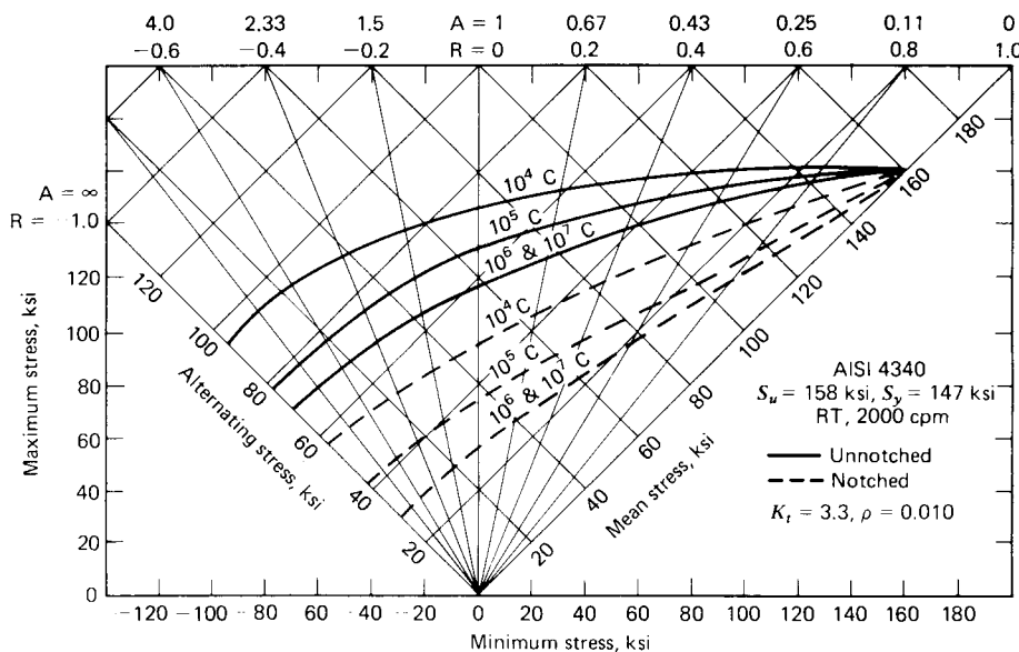
Fig. 20 Master diagram for 4340 steel. (From Ref. 24, p. 37.)
