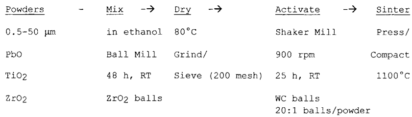
Fig. 4 Schematic flowchart for mechanochemical processing of PZT.
