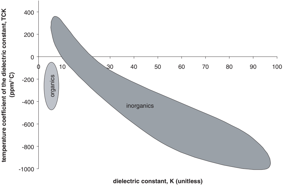
Fig. 16 Harrop correlation for dielectric materials.
