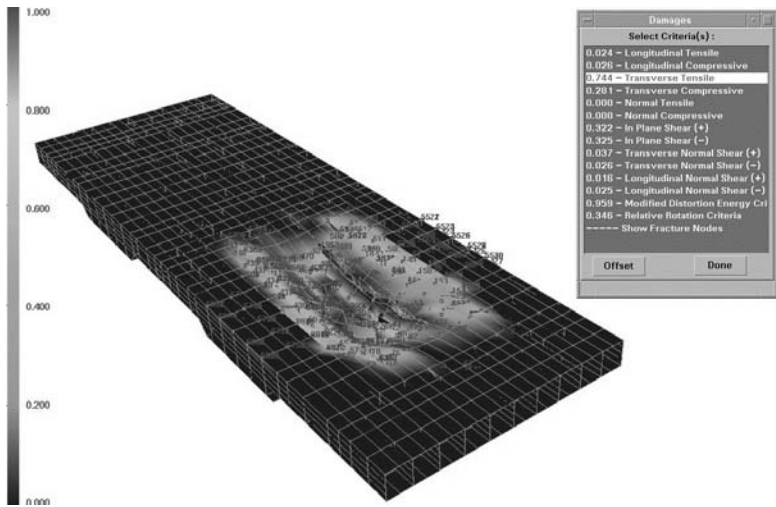
Fig. 55 Full-scale simulated destructive test using GENOA Progressive failure program. (Courtesy of Alpha Star Corporation, Long Beach, California)
