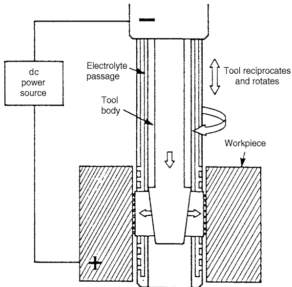
Fig. 42 Electrochemical honing.
