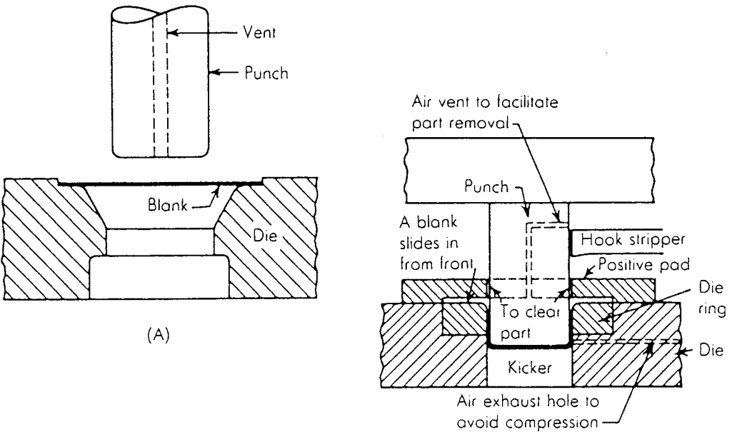
Fig. 8 Drawing process.
