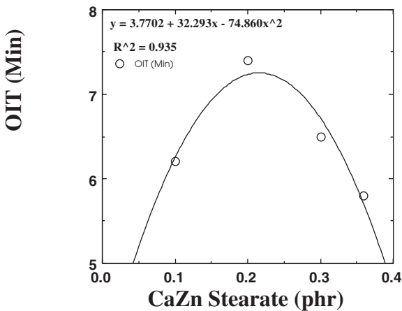
Fig. 1 PVC OIT dependence on CaZn stearate.
