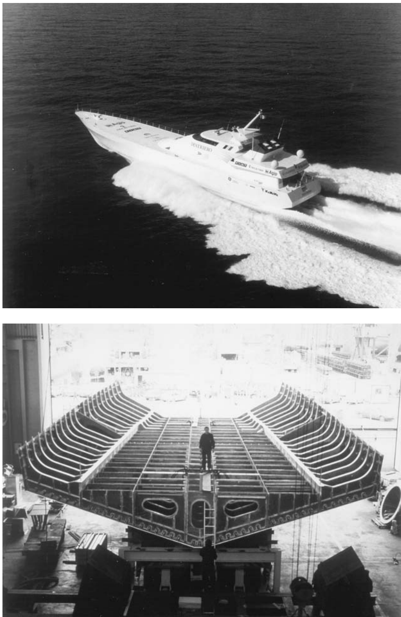
Fig. 11 High-speed single-hull ships (a) like the Proserpio employ 5083 or 5383-H113/H321 machined plate for hulls, (b) internal hull stiffeners, decking, and superstructure.
